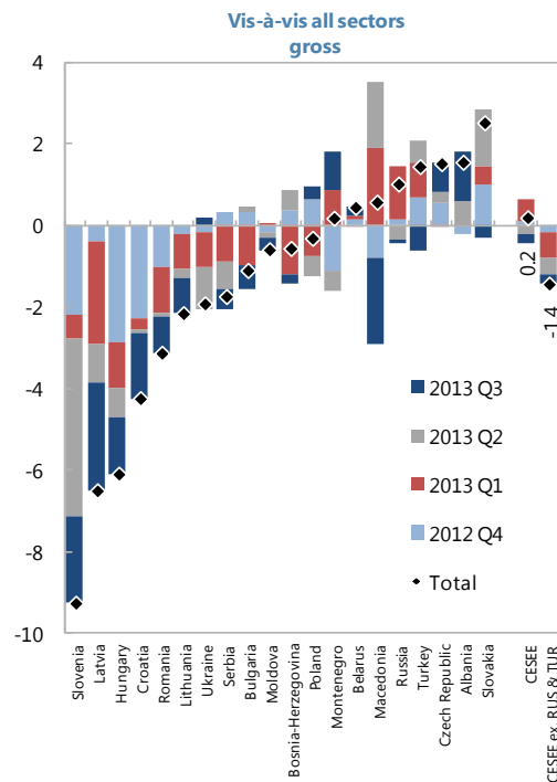
Figure 3. CESEE: External Positions of BIS-reporting Banks, 2012:Q4-2013:Q3 (Change, percent of 2013 GDP, exchange-rate adjusted)
